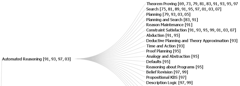
(a) A partial structure of levels 2 and 3 in the Artificial Intelligence Ontology
