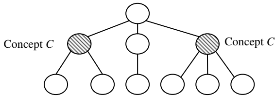
Fig. 7. Situation II: Concept duplication with shared super class
