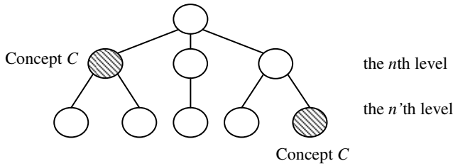
Fig.10. Situation IV: Concept duplication with different super class and located in different levels
