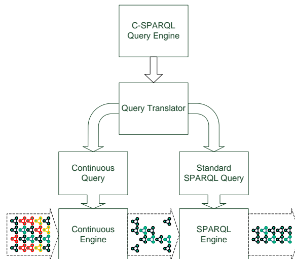
Figure 2.1: High level architecture of a C-SPARQL engine
