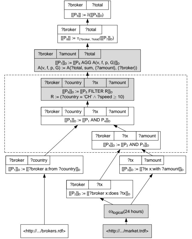
Figure 1: O-Graph of the example query
