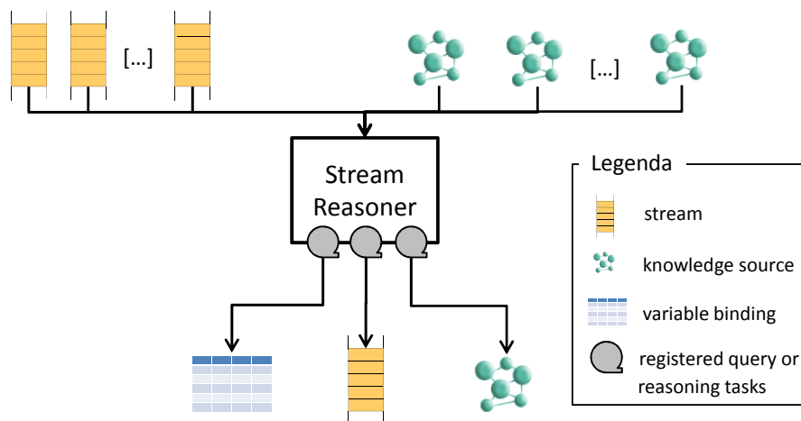
Figure 2.2: Inputs and output of a C-SPARQL Engine
