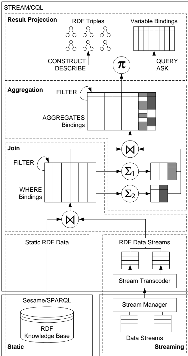
Figure 4: Query evaluation process
