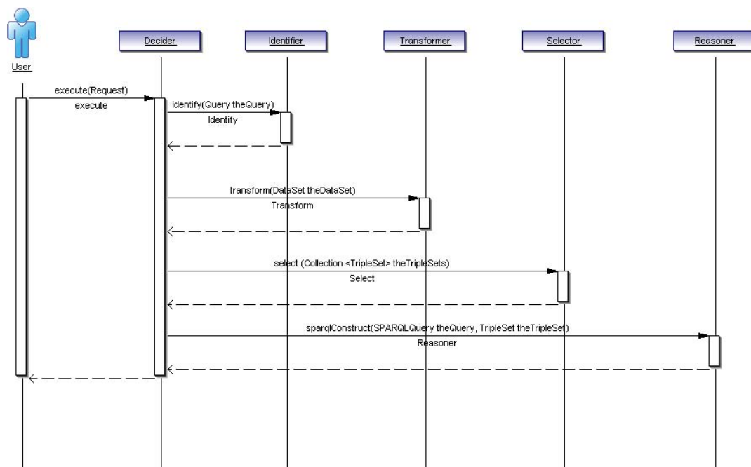
Figure 3.2: UML sequence diagram describing a possible interaction of plug-ins to implement the use case
